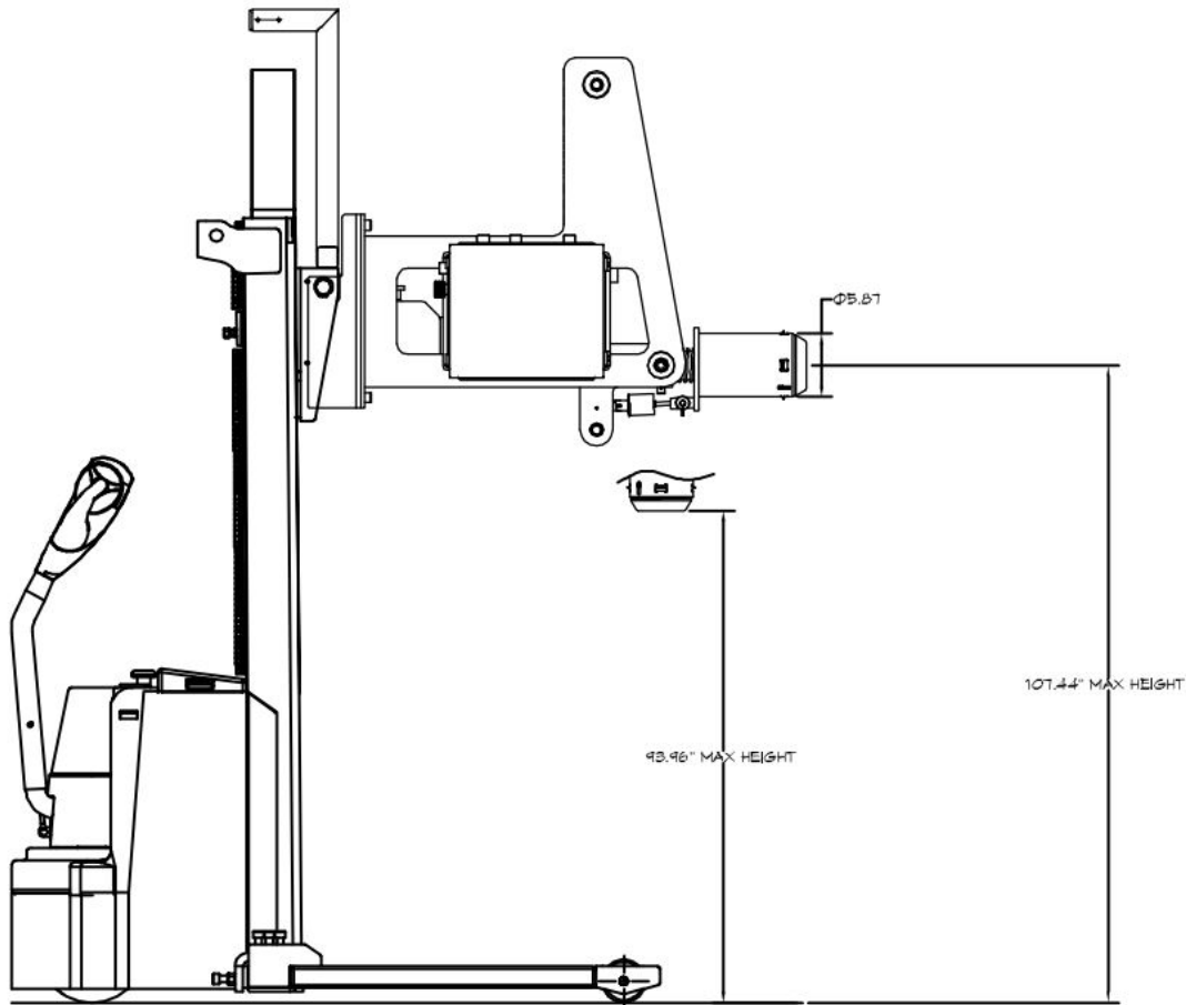
Dimensions show with PPS2200-101
